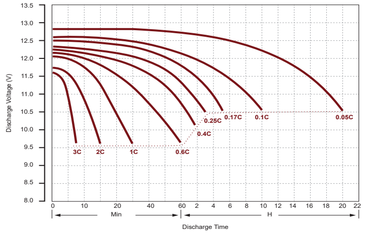
Discharging Characteristic (25°C)
