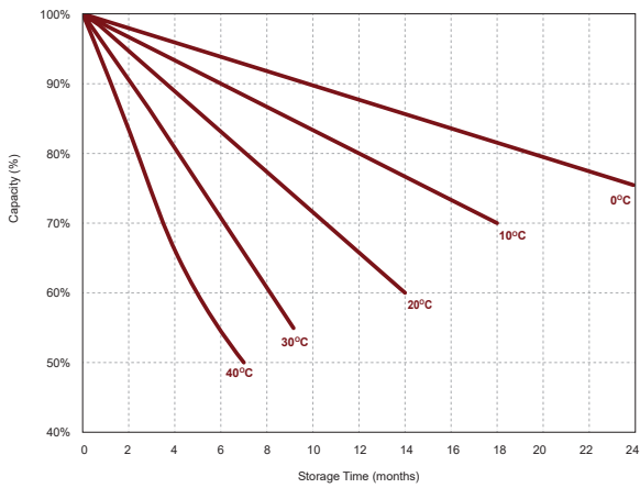
Self-Discharge Characteristics
