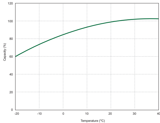
The Effect of Temperature on Capacity
